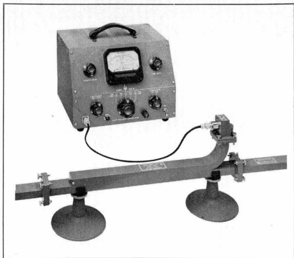
Fig. 1. New -hp- Model 487A broadband thermistor mount used with directional coupler and power meter to monitor power level in waveguide system.
