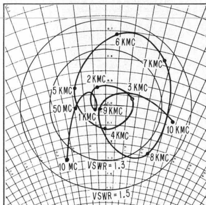
Fig. 6. Typical admittance characteristic of -hp- Model 477A coaxial thermistor mount.
