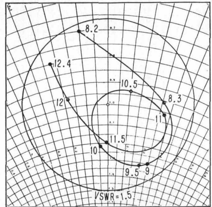
Fig. 4. Typical impedance characteristic of waveguide thermistor mount for 8.2 to 12.4 kmc range (Model X487A).
