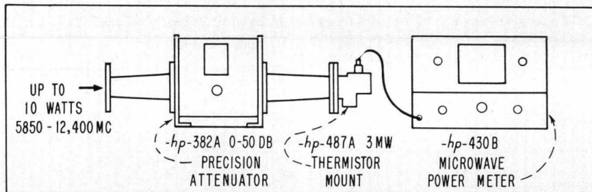
Arrangement for measuring average powers up to 10 watts in waveguide systems. See note above concerning attenuators.
