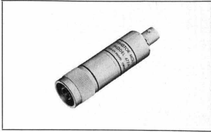
Fig. 5. -hp- Model 477A coaxial thermistor mount for use from 10 mc to 10 kmc.
