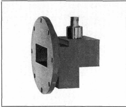
Fig. 2. Model 487A waveguide mount for use with 2" x 1" waveguide from 3.95 to 5.85 kmc.
