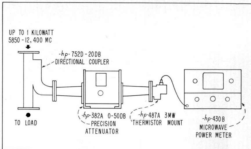
Arrangement for monitoring average powers up to 1 kilowatt in waveguide systems. -hp- Model 750D series cross-guide directional couplers may be used in place of Model 752D. See note above concerning attenuator. For monitoring coaxial systems, -hp- 281A series coax-waveguide transitions can be used at each end of directional coupler.
